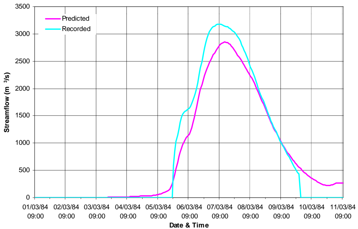
Figure A.3 Recorded and Predicted Discharges, URBS Model, Katherine River at Gorge Caravan Park (G8140023), March 1984 Event
