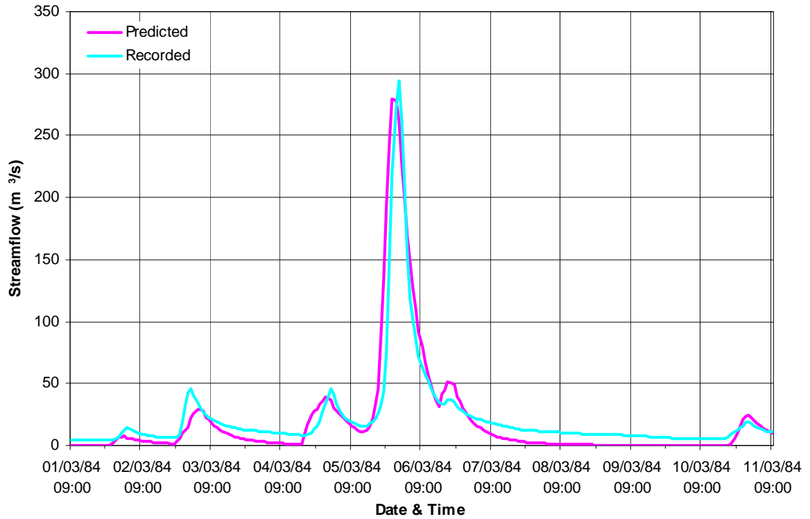
Figure A.5 Recorded and Predicted Discharges, URBS Model, McAdden Creek (G8140158), March 1984 Event
