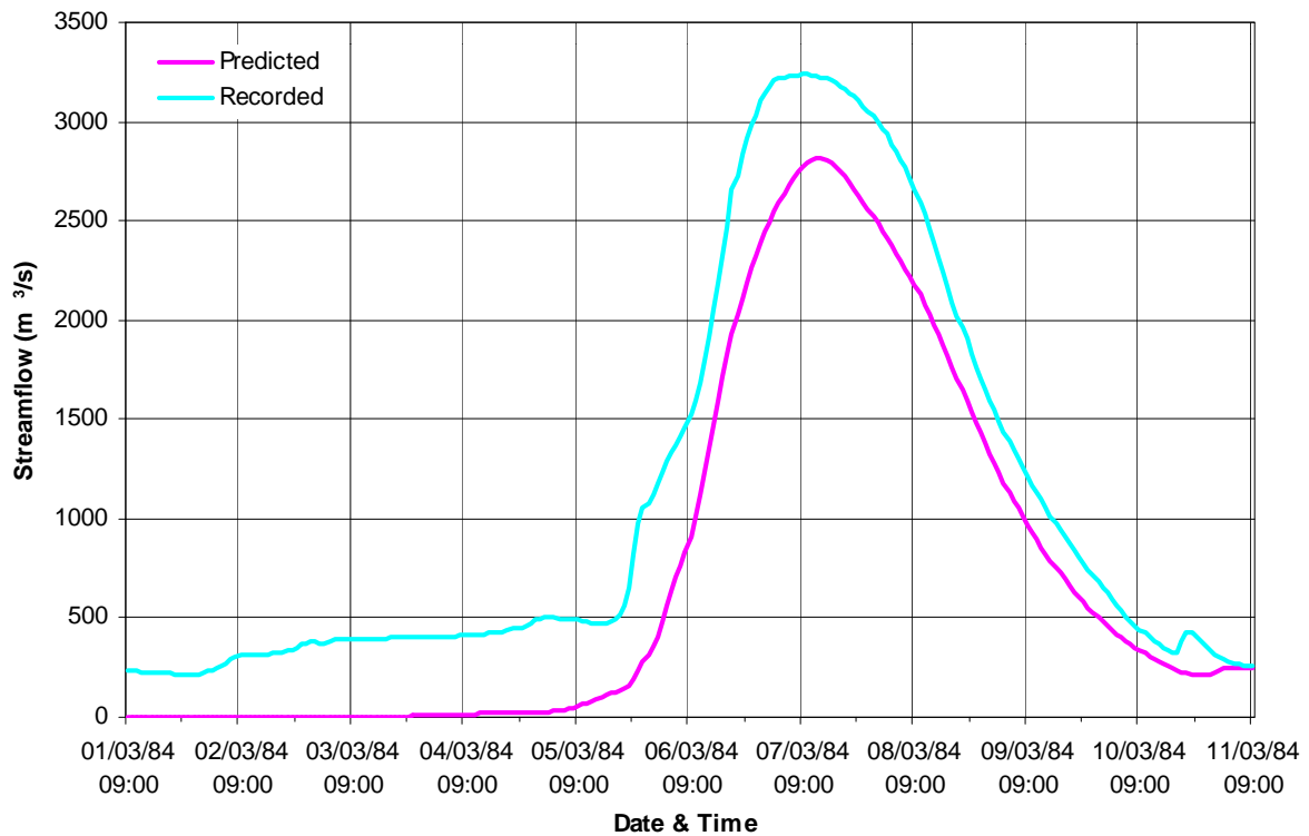
Figure A.2 Recorded and Predicted Discharges, URBS Model, Katherine River at Katherine Gorge (G8140019), March 1984 Event
