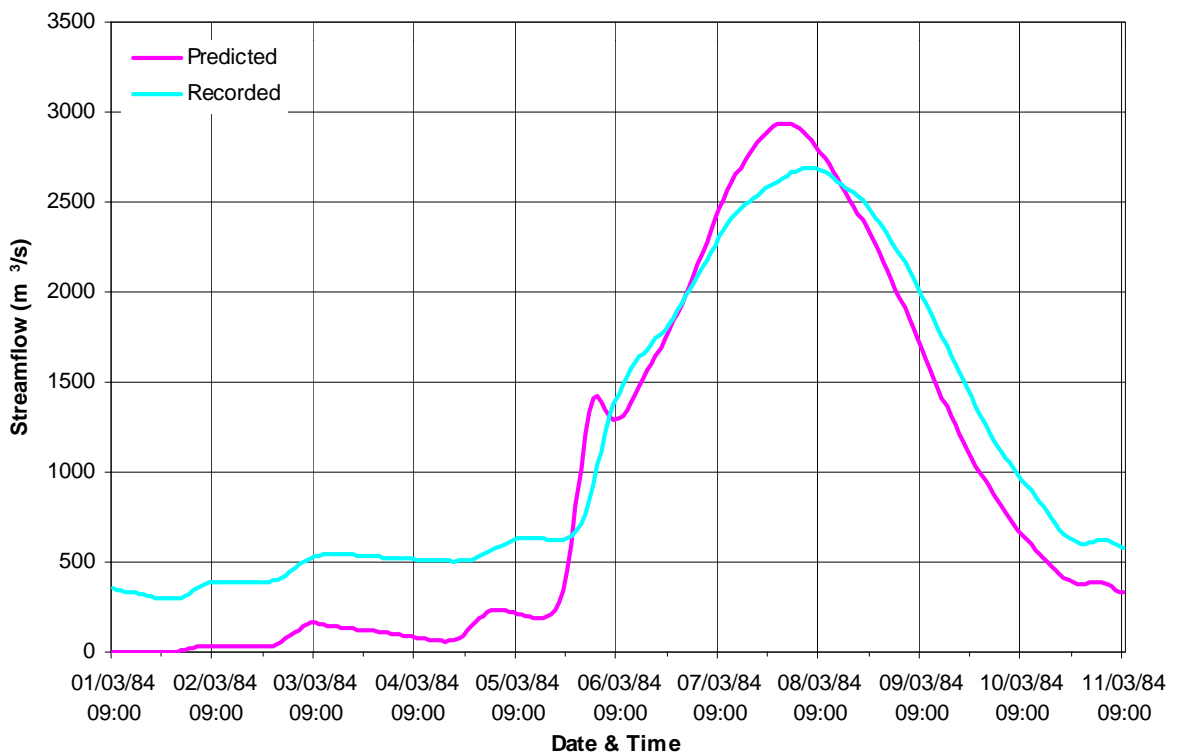
Figure A.6 Recorded and Predicted Discharges, URBS Model, Katherine River at Railway Bridge (G8140001), March 1984 Event
