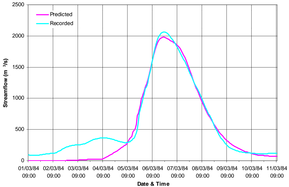
Figure A.1 Recorded and Predicted Discharges, URBS Model, Katherine River at Mt Ebsworth (G8140218), March 1984 Event
