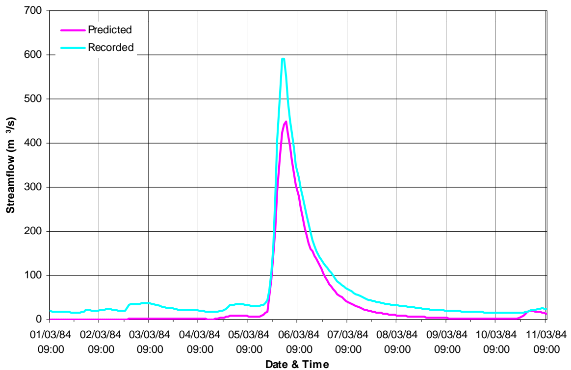
Figure A.4 Recorded and Predicted Discharges, URBS Model, Seventeen Mile Creek (G8140159), March 1984 Event
