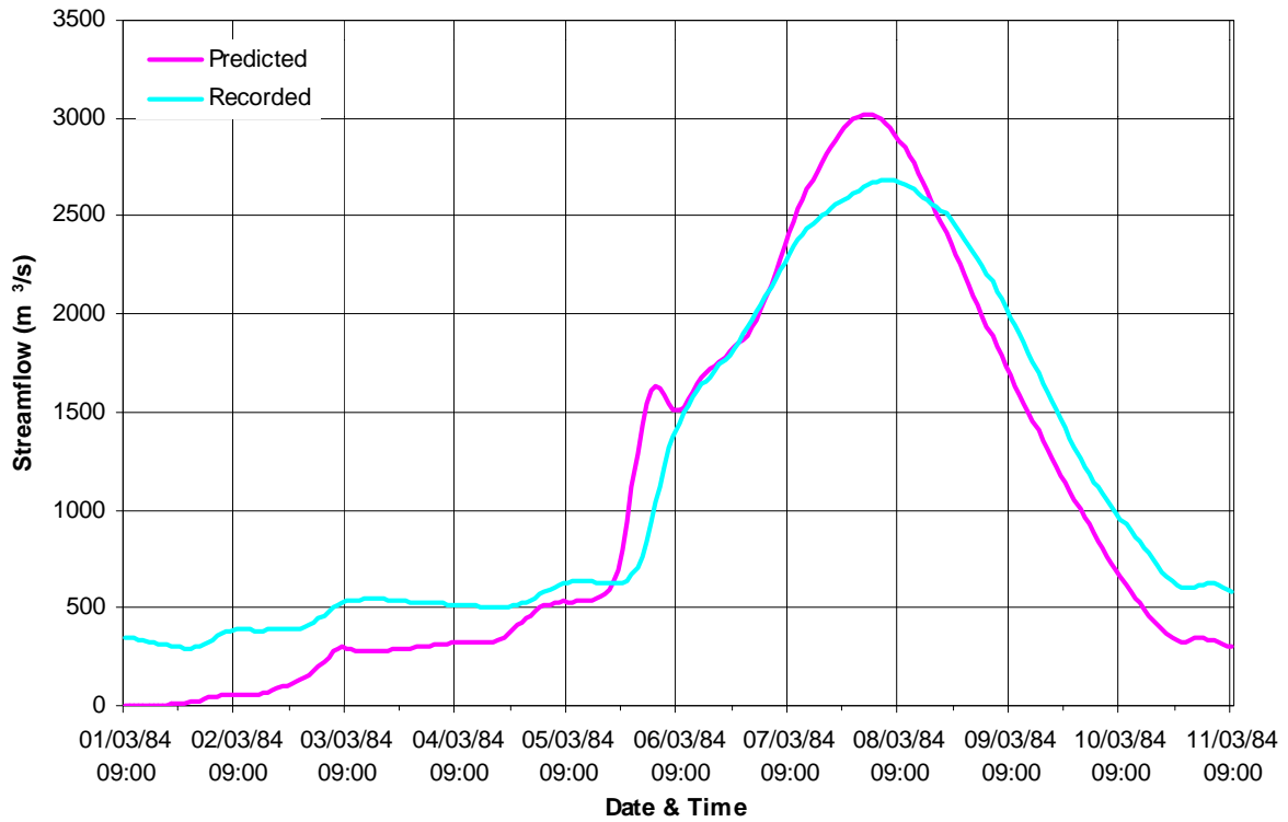
Figure A.7 Recorded and Predicted Discharges, URBS Model, Katherine River at Railway Bridge (G8140001), Matched Hydrographs at Seventeen Mile and McAdden Cks, March 1984 Event
